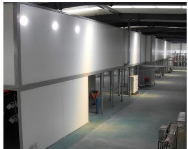
Tunnel type powder coating curing oven
